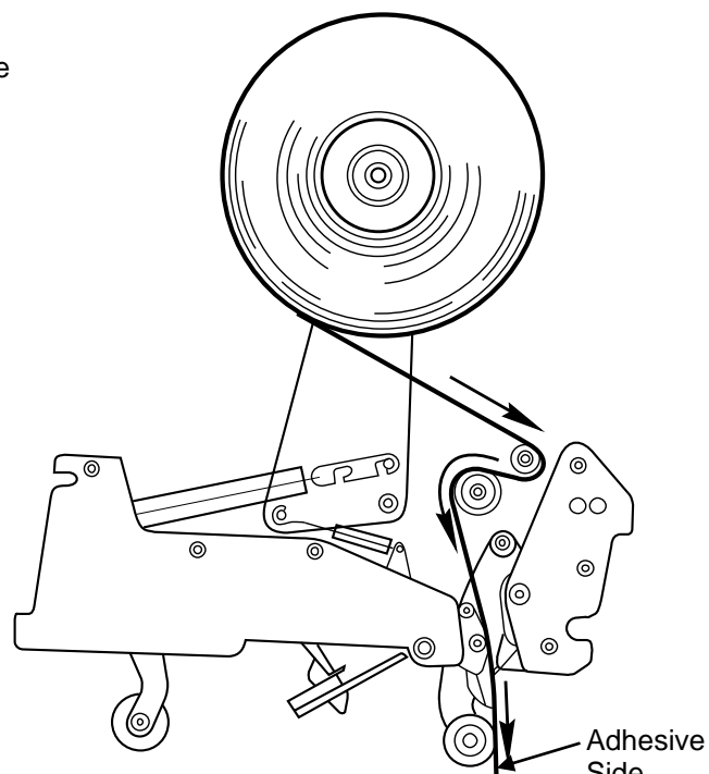
Upper Cartridge
