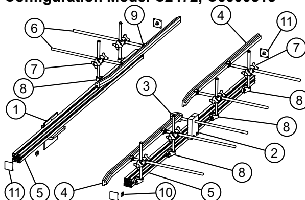
Bump Turn Retrofit Kit for Earlier Configuration Model C2472, C0000515
